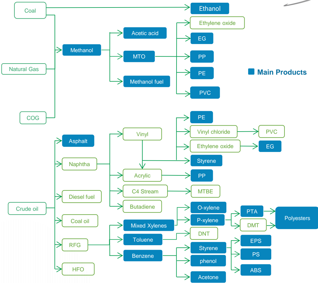
Petrochemicals Flowchart
