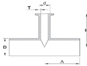
Automatic Tube Weld : Standard Outlet Hygienic Clamp Joint: Reducing Tee-ASME BPE -2022,DT-4.1.2-13
