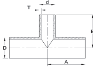
Automatic Tube Weld: Reducing Tee-ASME BPE -2022,DT-4.1.2-6
