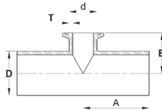
Automatic Tube Weld: Short Outlet Hygienic Clamp Joint Reducing Tee-ASME BPE -2022,DT-4.1.2-7
